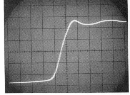
Fig. 4. Very fast sweep speed of 0.1 nsec/cm shows low trigger-to-pulse jitter of 213B Generator when triggered by -hp- 185B Sampling Oscilloscope. Oscilloscope sampled several hundred pulses during exposure to display leading edge. Apparent risetime of step includes finite scope risetime.
