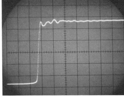
Fig. 3. Sweep speed of 0.5 nsec/cm shows very fast rise of -hp- 213B Pulse Generator output. Minimum-length signal paths were used in observation set-up, although it is quite small for such a fast step.
