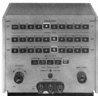
Fig. 4. Photograph indicating method of selecting output frequency in new oscillator. Buttons are set to give output frequency of 455 kc.
